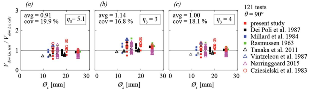
Fig. 81 Comparison of Rasmussen's model with the considered database of dowel tests with \theta = 90^\circ .
