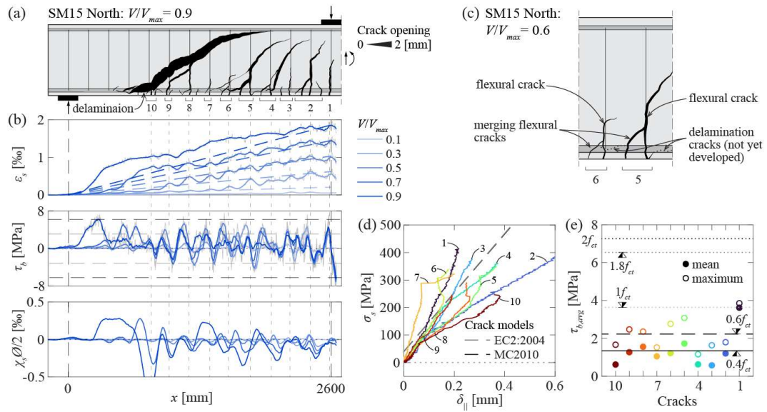
Fig. 38 Detailed crack results of the flexural reinforcement from the North face of specimen SM15: (a) crack pattern for V/V_{max} = 0.9 ; (b) steel strain, bond stress and normalized curvature distributions for five load levels; (c) contribution of the secondary cracks to the crack width for cracks 5 and 6; (d) rebar stress – crack width diagrams for all cracks; and (e) mean and maximum values of the average bond stress at both sides of the crack (in the range between \delta_{||} \geq 0.1 mm and \sigma_s < 500 MPa).
