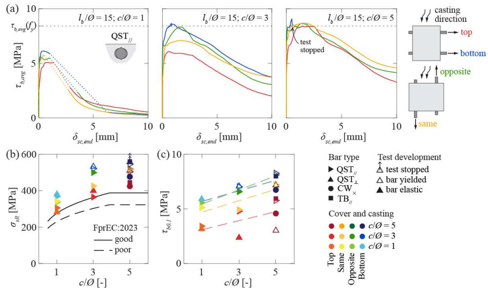
Fig. 24 Effect of concrete cover and casting conditions: (a) average bond stress-slip relationships for specimens with covers of 1Ø (PC0201, 03, 13 and 16), 3Ø (PC0205, 07, 14 and 17) and 5Ø (PC0209, 11, 15 and 18); (b) anchorage resistance as a function of concrete cover; and (c) average bond stress corresponding to a slip at the unloaded end of 0.1 mm as a function of concrete cover.
