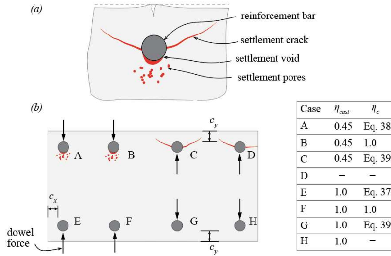
Fig. 69 (a) Consequences of settlement and bleeding of fresh concrete around top bars (adapted from Moccia et al. [224]); and (b) investigated cases and proposed coefficients \eta_c (influence of cover) and \eta_{cast} (influence of casting condition).
