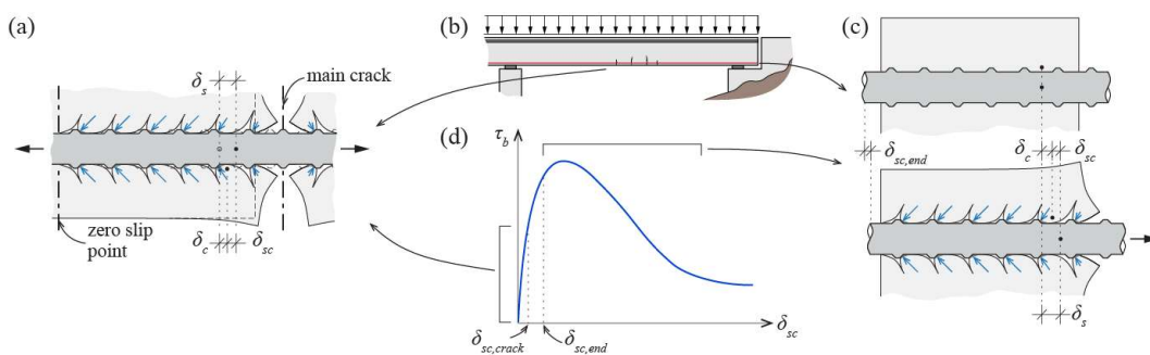
Fig. 18 Bond in structural members; schematic representation of (a) a cracked region, (b) a reinforced concrete beam and (c) an end anchorage; and (d) general bond-slip relationship.
