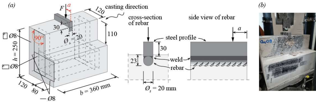
Fig. 48 Specimens for CP tests: (a) geometry, reinforcement and applied force and (b) photo of a specimen.
