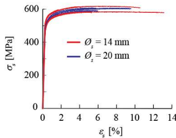
Fig. 49 Stress-strain relationships of the reinforcement.
