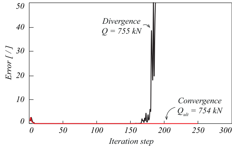
Fig. 18 Convergence and divergence of a JCONC simulation
