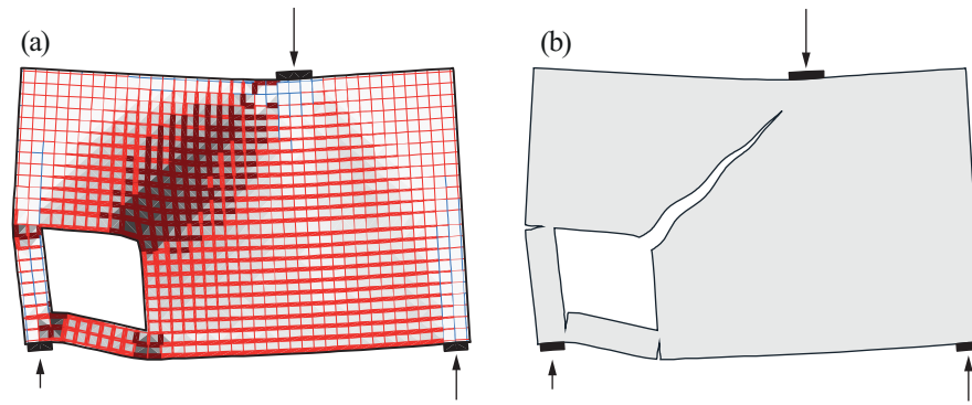
Fig. 6 Licit failure mechanism: obtained using EPSF method (a); obtained using RPSF method (b)
