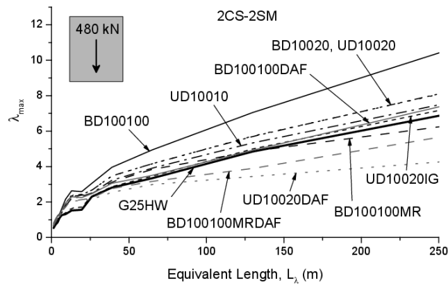
(b) Second support moment of two-span continuous bridge
