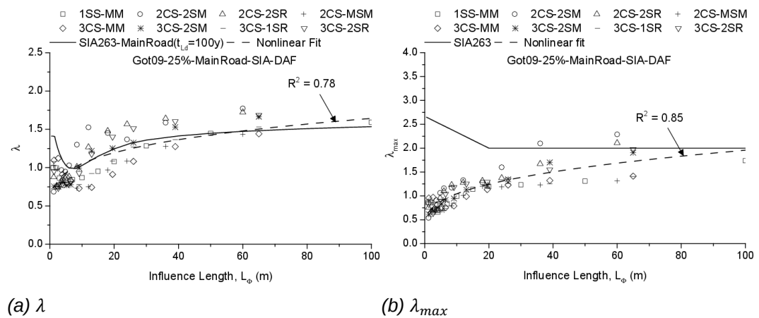
Fig. IV.6 SIA-base damage equivalence factors for G25MRDAf traffic
