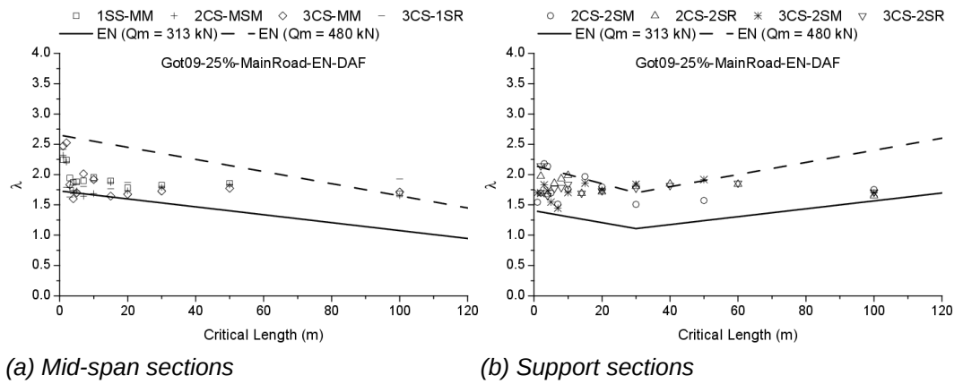
Fig. IV.12 Eurocode-base \lambda for G25MRDAF traffic
