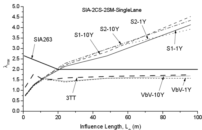
(b) two-span continuous bridge - second support moment
