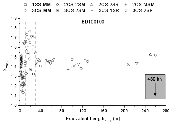
(a) bidirectional traffic, BD100100
