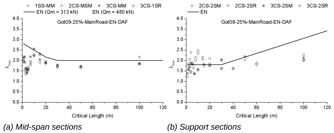
Fig. IV.18 Eurocode-base \lambda_{max} for G25MRDAF traffic
