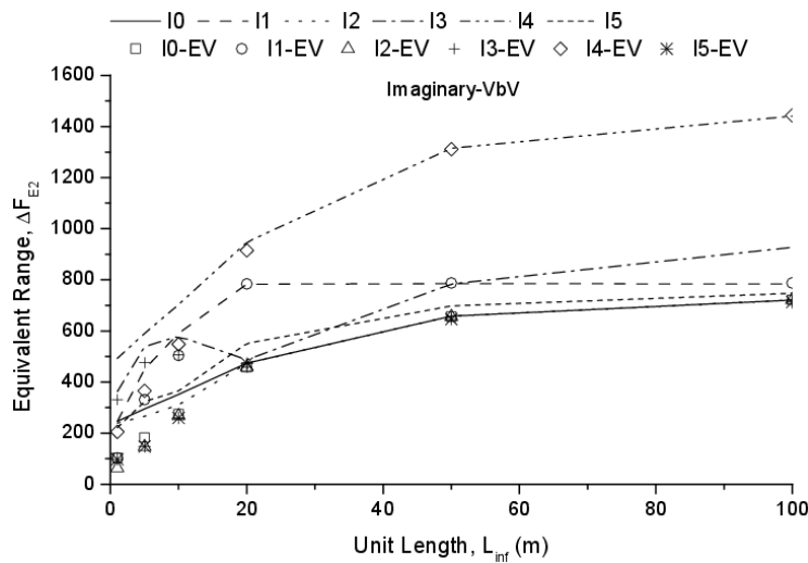
Fig. 4.7 Equivalent force range estimated by equivalent vehicle in comparison with simulation results
