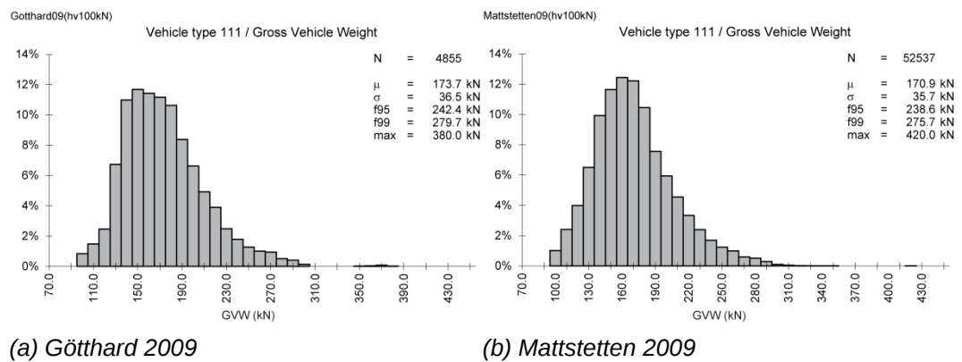
Fig. III.8 Frequency of GVW for truck Type 111
