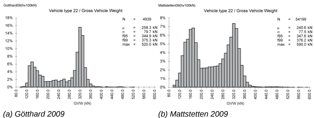
Fig. III.6 Frequency of GVW for truck Type 22
