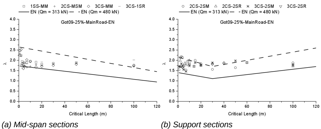
Fig. IV.9 Eurocode-base \lambda for G25MR traffic
