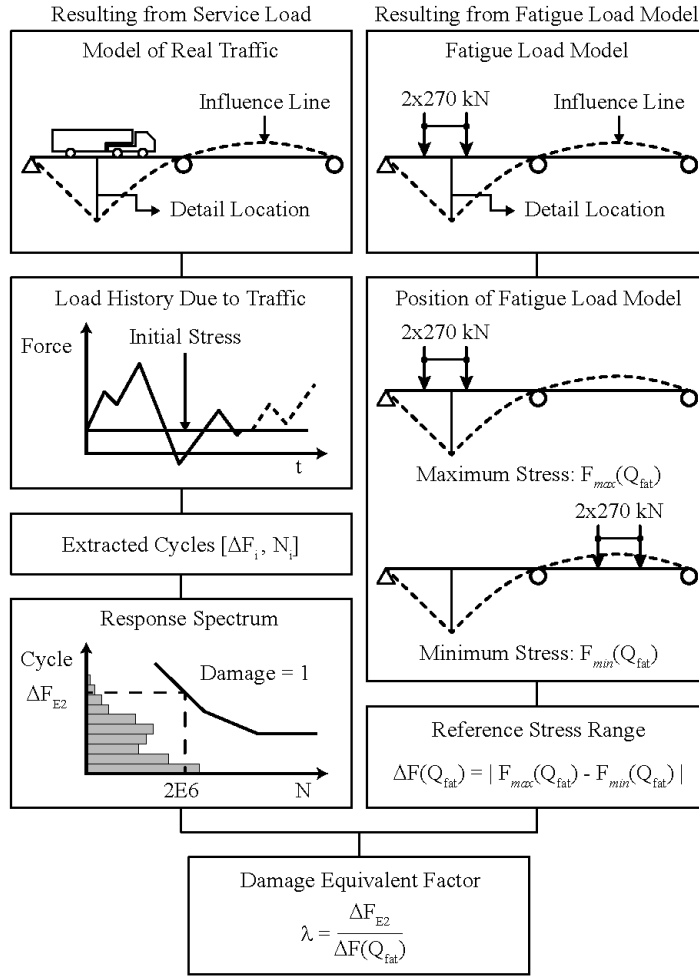
Fig. 3.1 Concept of damage equivalence factor
