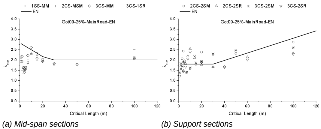
Fig. IV.15 Eurocode-base \lambda_{max} for G25MR traffic
