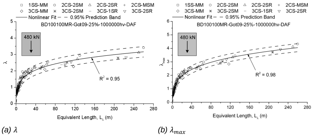
Fig. IV.33 \lambda and \lambda_{max} based on the proposed method obtained for BD100100MRDAF traffic
