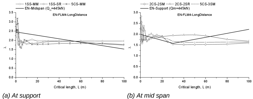
Fig. II.5 Comparison of \lambda with FLM4 for long distance traffic
