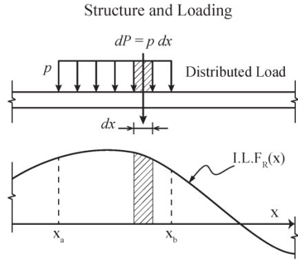
Fig. 4.9 Parameters for finding maximum response due to uniformly distributed load
