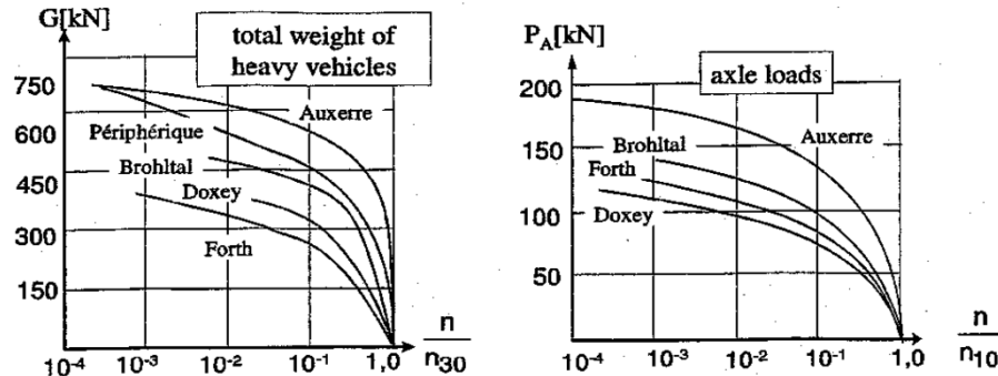
Fig. 5.6 Accumulated distribution of GVW and axle load at various European stations [77]
