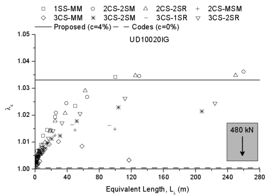
Fig. IV.39 \lambda_4 based on the proposed method for UD10020IG traffic
