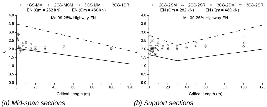
Fig. IV.10 Eurocode-base \lambda for M25HW traffic
