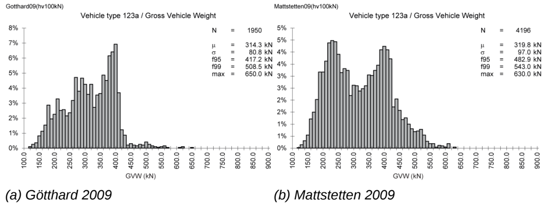
Fig. III.13 Frequency of GVW for truck Type 123a
