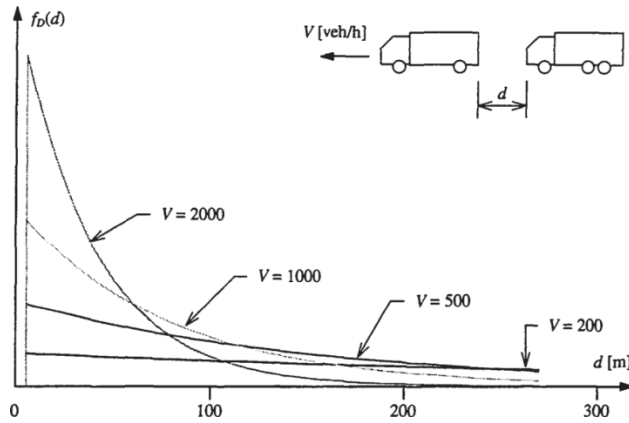
Fig. 2.8 Distance between vehicles in free-moving traffic [7]
