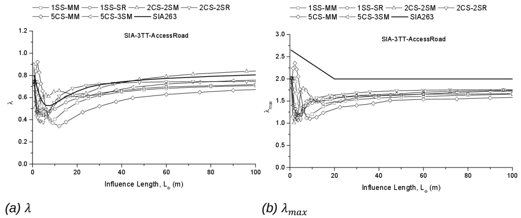
Fig. II.4 \lambda and \lambda_{max} obtained from 3TT for access road traffic in comparison with SIA263
