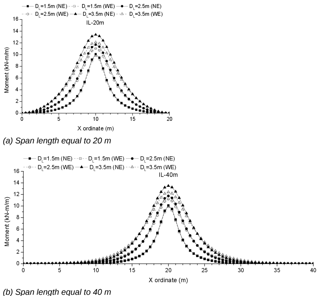
Fig. 4.22 Transversal moment of cantilever slab according to lane position
