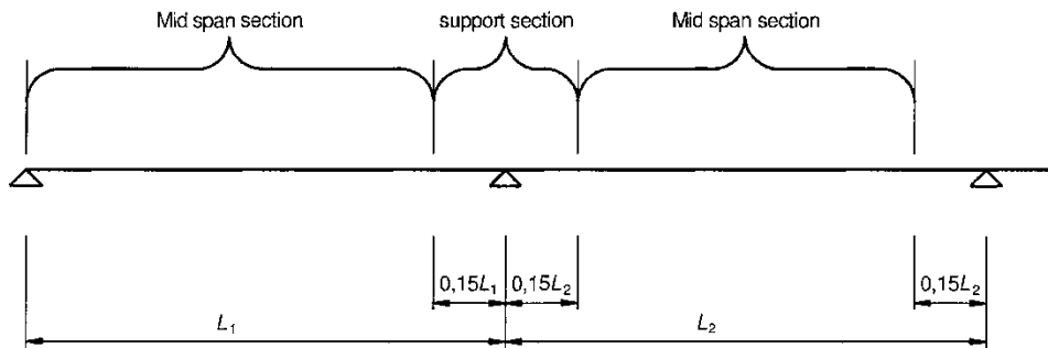
Fig. 3.9 Eurocode definition for location of mid span and support section zones [27]
