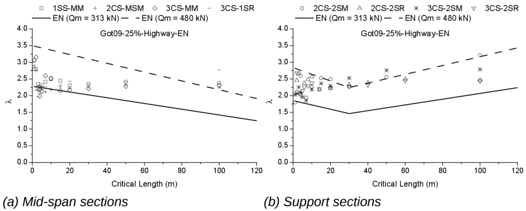
Fig. IV.8 Eurocode-base \lambda for G25HW traffic
