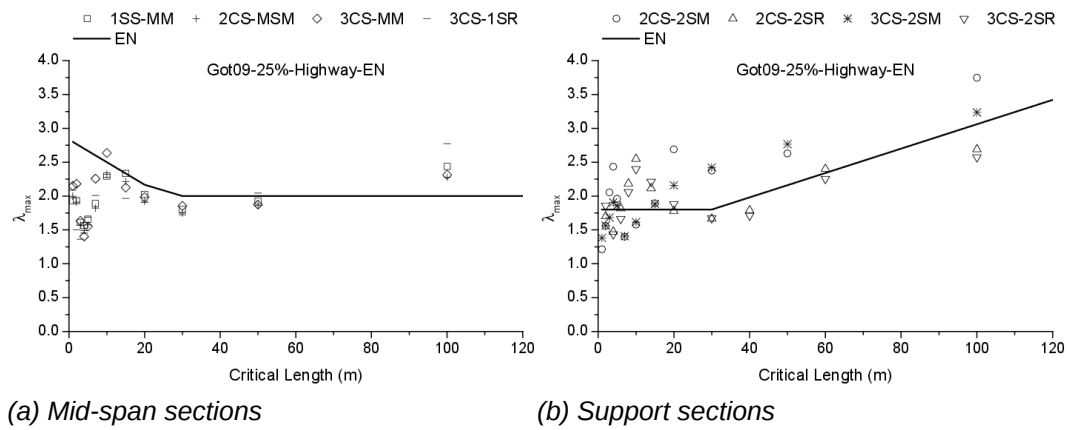
Fig. IV.14 Eurocode-base \lambda_{max} for G25HW traffic
