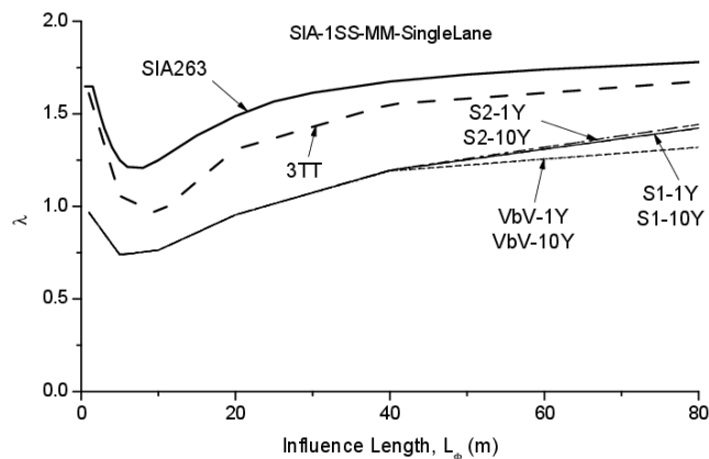
(a) Mid moment of simple-span bridges
