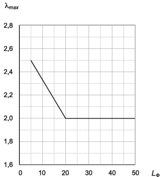
Fig. 3.4 \lambda_{max} for roadway bridges based on SIA263 [81]
