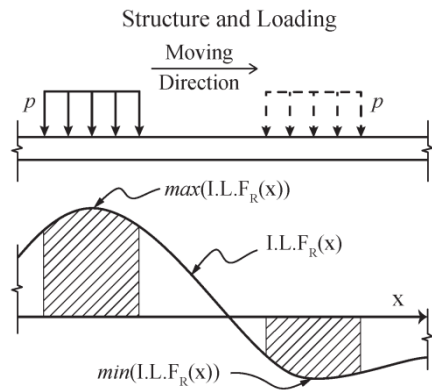
Fig. 4.10 Parameters for finding force range due to passage of uniformly distributed load with a defined length
