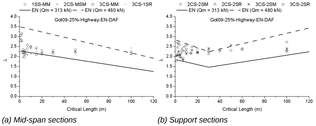
Fig. IV.11 Eurocode-base \lambda for G25HWD AF traffic
