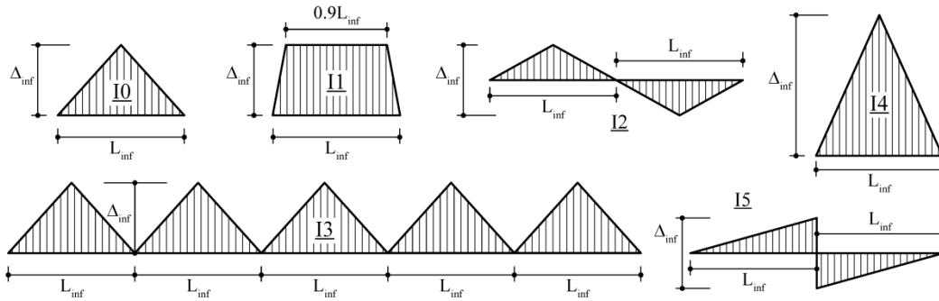
Fig. 4.2 Shape of imaginary influence lines
