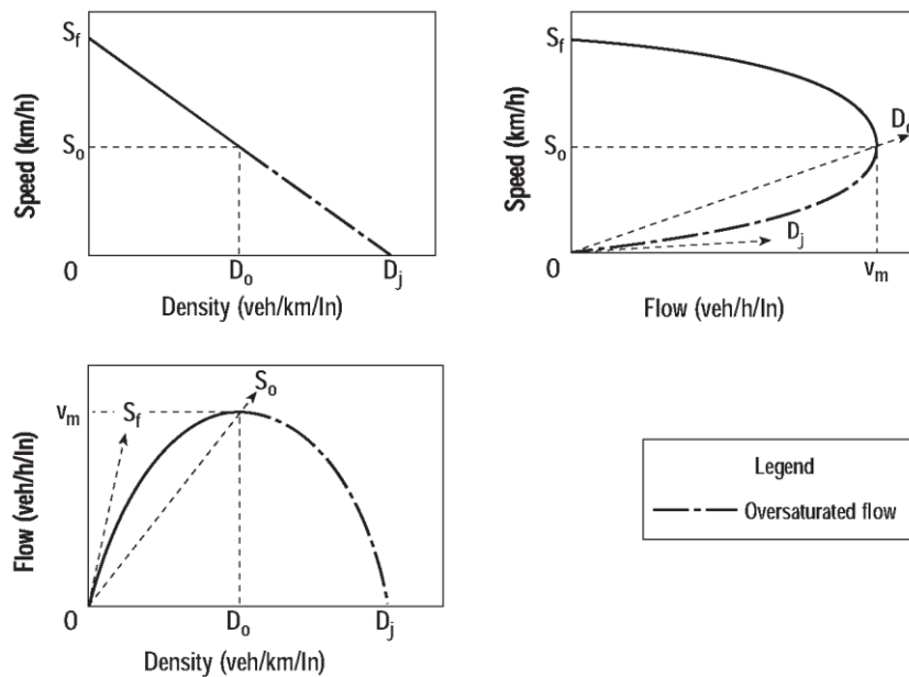
Fig. 2.7 General relationships among speed, density and flow rate [39]
