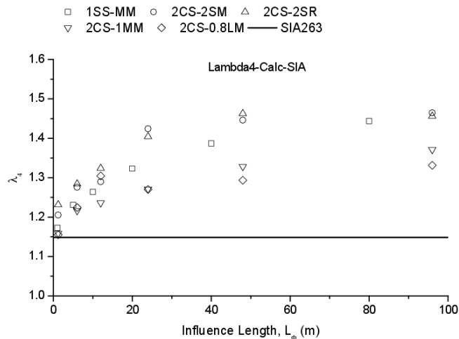
(a) Bidirectional traffic 50-50 percent
