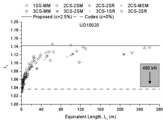
Fig. IV.37 \lambda_4 based on the proposed method for UD10020 traffic
