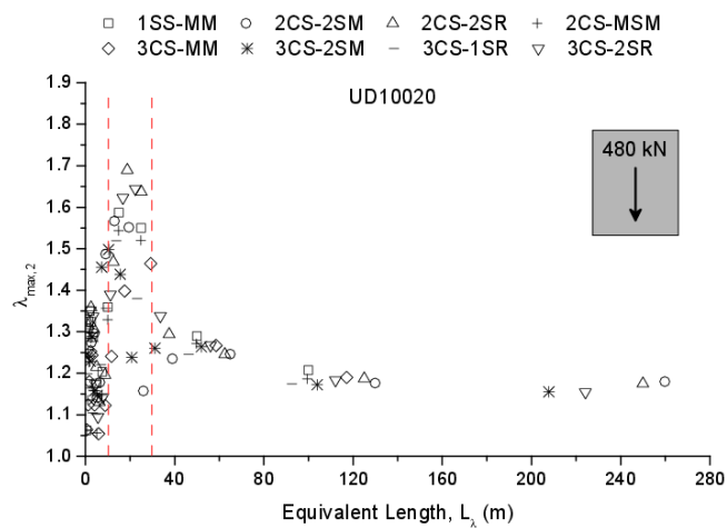
(b) unidirectional traffic, UD10020
