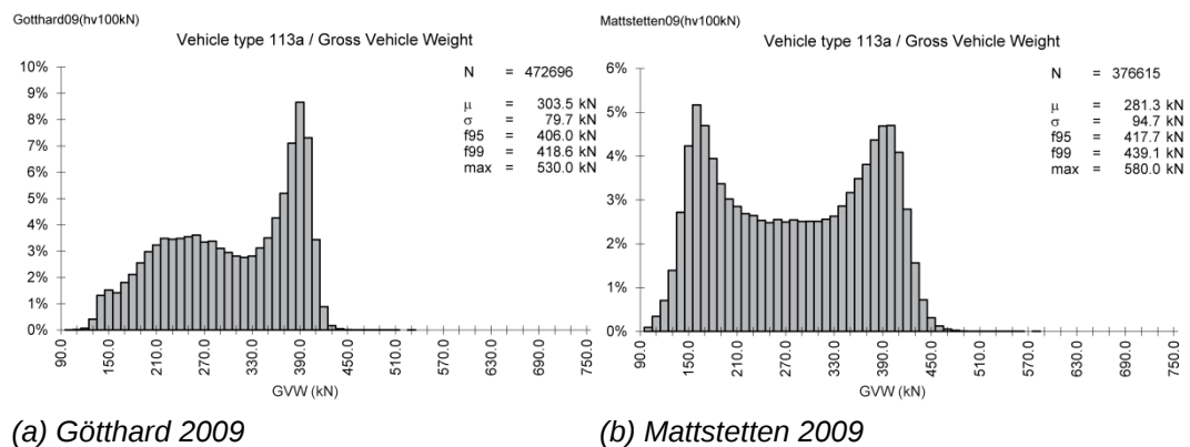
Fig. III.11 Frequency of GVW for truck Type 113a
