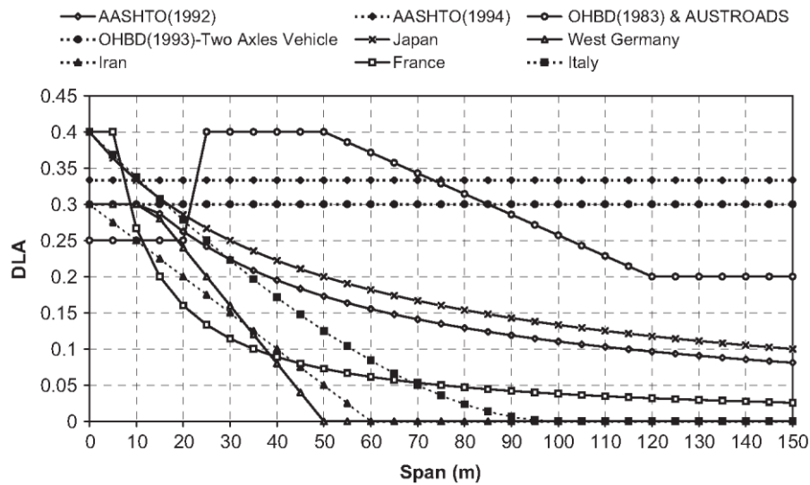
Fig. 2.14 dynamic load allowance based on various design codes [64]
