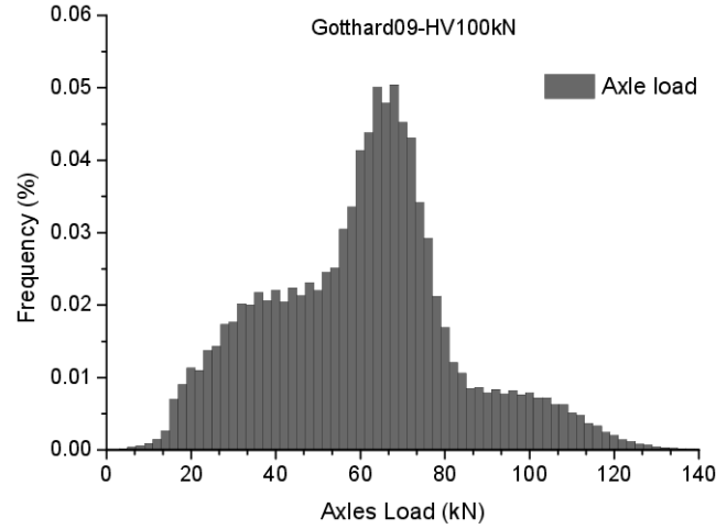
(a) Axle load
