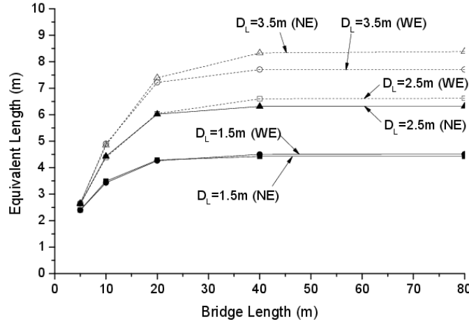
Fig. 4.23 Relation between fatigue equivalent length and bridge length
