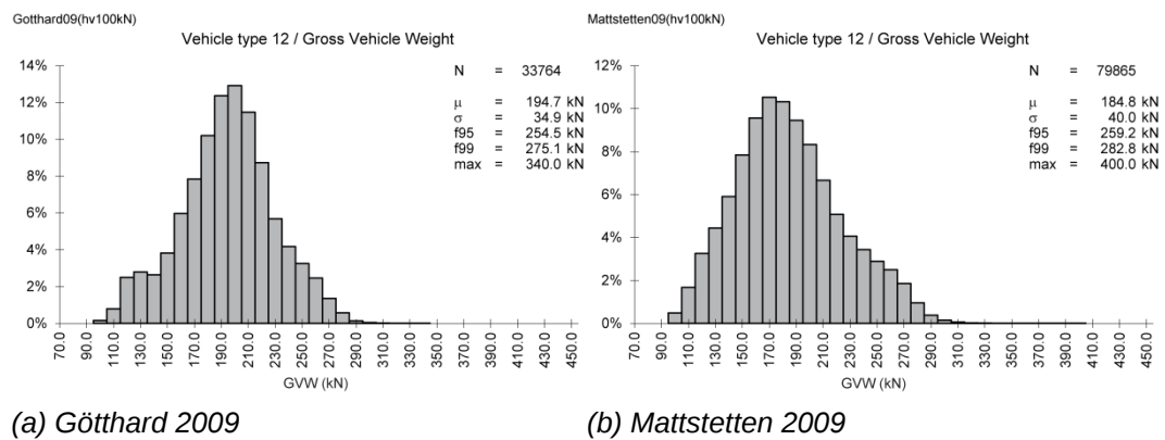
Fig. III.5 Frequency of GVW for truck Type 12
