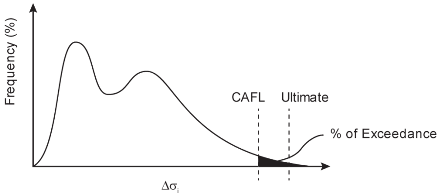
Fig. 4.18 Schematic diagram of bridge response cycles frequency due to traffic
