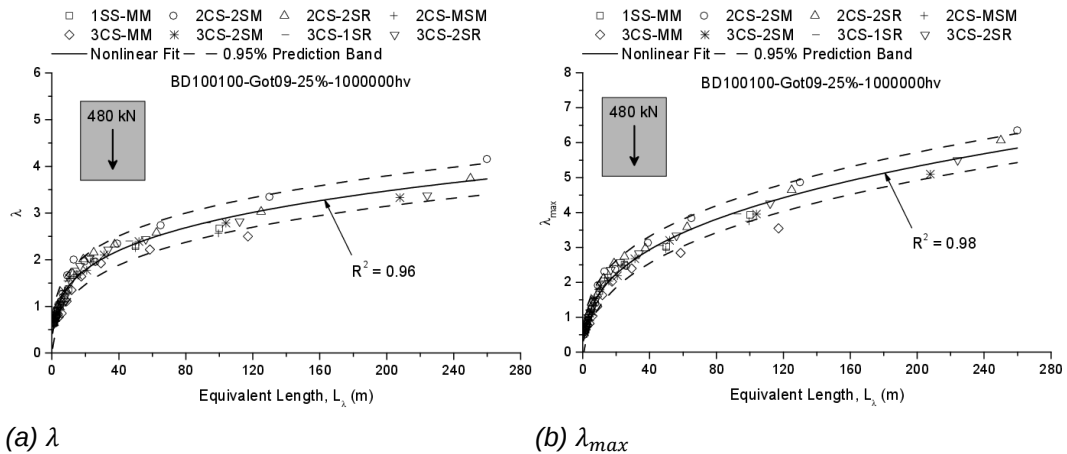
Fig. IV.27 \lambda and \lambda_{max} based on the proposed method obtained for BD100100MR traffic
