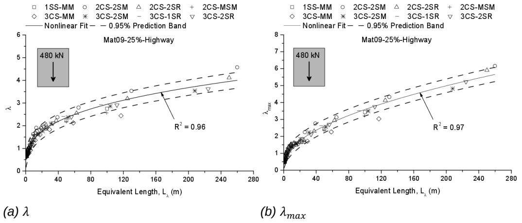
Fig. IV.22 \lambda and \lambda_{max} based on the proposed method obtained for M25HW traffic
