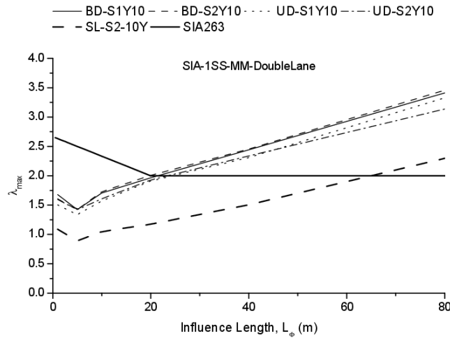
(a) Simple-span bridge - mid moment
