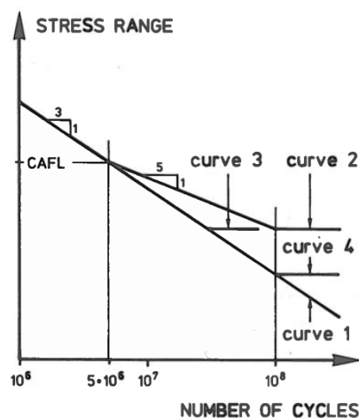
Fig. 2.4 The different fatigue S-N curves examined by Smith et al. [84]
