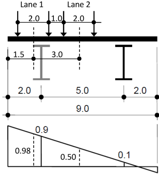
Fig. 3.3 Example of transverse distribution of two-girder bridge cross section in function of lateral load positions
