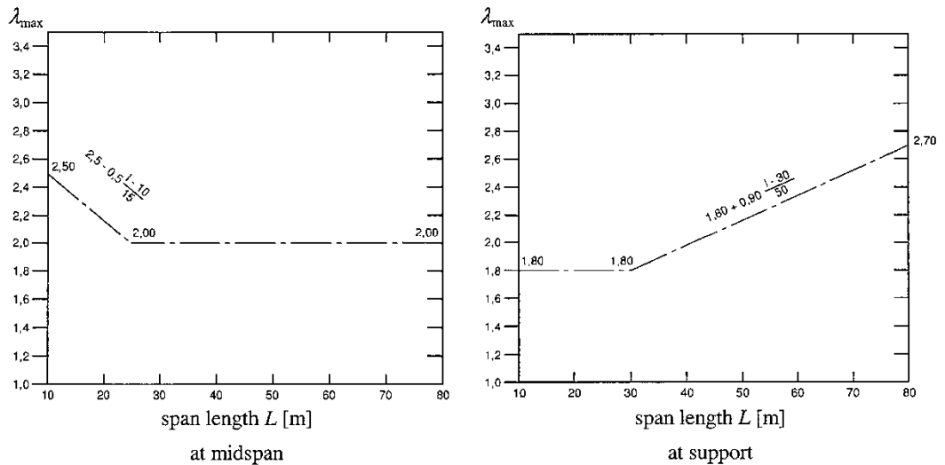
Fig. 3.10 \lambda_{max} for roadway bridges based on EN1993-2 [27]
