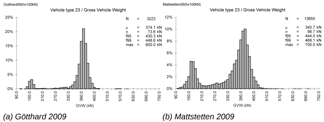
Fig. III.7 Frequency of GVW for truck Type 23
