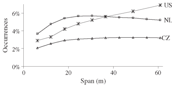
Fig. 2.11 Multiple presences of trucks with one truck in each lane [69]
