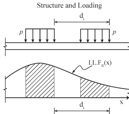
Fig. 4.13 Parameters for finding force range due to passage of two following vehicles
