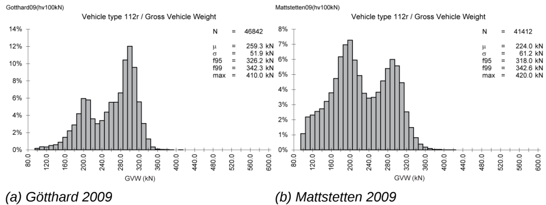
Fig. III.10 Frequency of GVW for truck Type 112r
