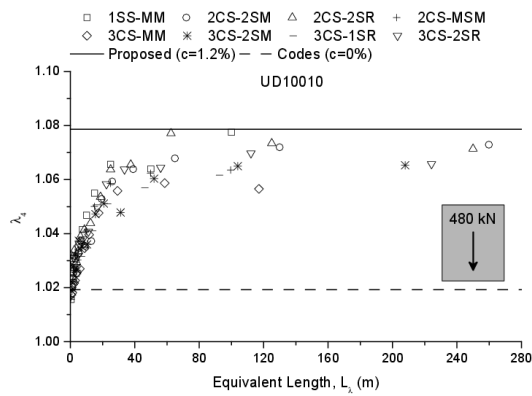
Fig. IV.38 \lambda_4 based on the proposed method for UD10010 traffic
