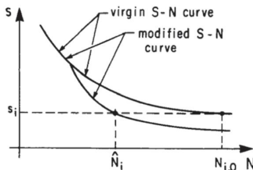
Fig. 2.1 Schematic representation of the modified S-N curve according to the Leipholz approach [50]
