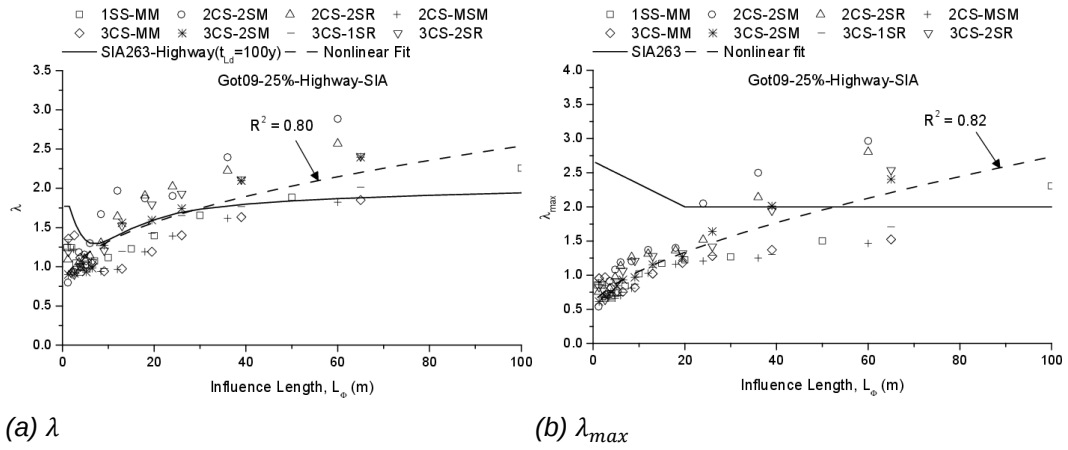
Fig. IV.2 SIA-base damage equivalence factors for G25HW traffic
