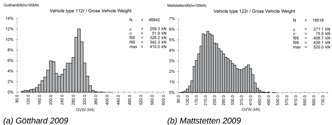
Fig. III.12 Frequency of GVW for truck Type 122r
