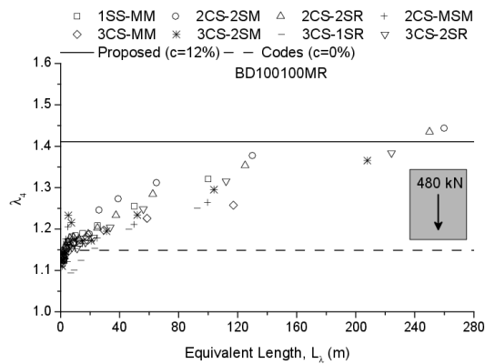
Fig. IV.36 \lambda_4 based on the proposed method for BD100100MR traffic
