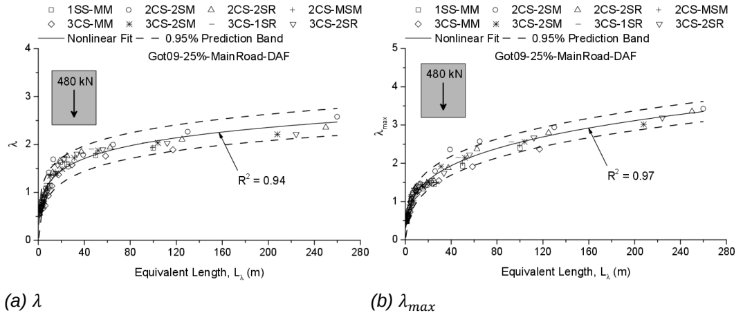
Fig. IV.24 \lambda and \lambda_{max} based on the proposed method obtained for G25MRDAF traffic
