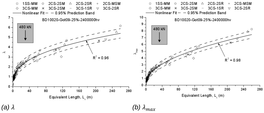
Fig. IV.25 \lambda and \lambda_{max} based on the proposed method obtained for BD10020 traffic
