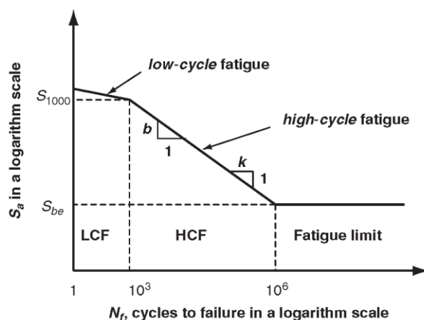
Fig. 2.2 A schematic S-N curve for steel [49]
