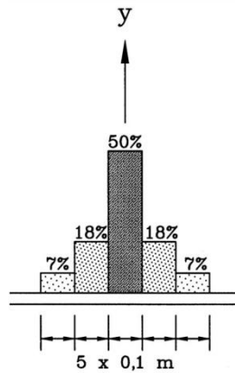
Fig. 4.24 Frequency distribution of transverse location of vehicles based on EN1991-2 [25]
