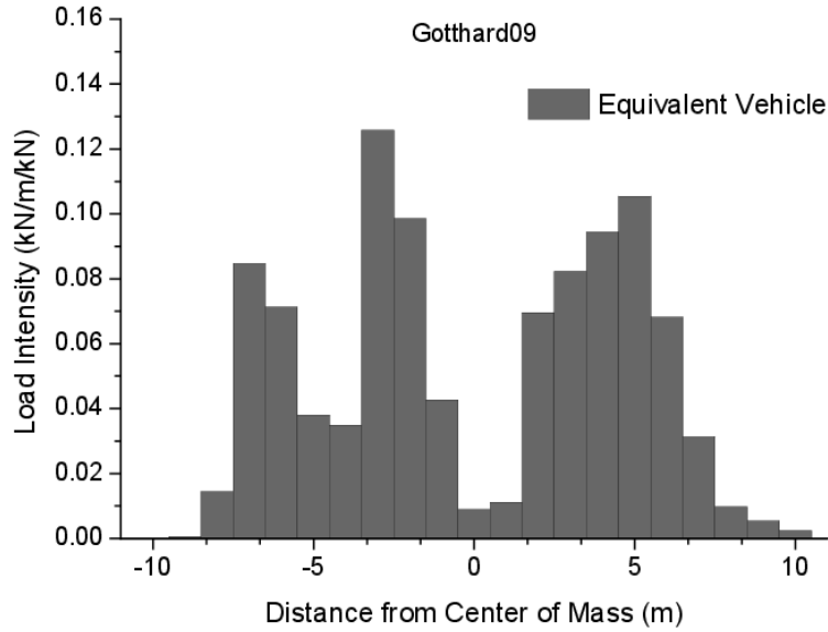
Fig. 4.6 Equivalent vehicle determined from the Götthard traffic in 2009
