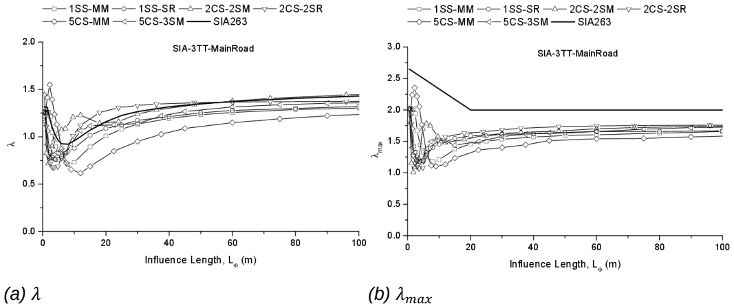
Fig. II.2 \lambda and \lambda_{max} obtained from 3TT for main road traffic in comparison with SIA263
