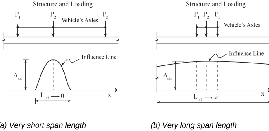
Fig. 4.4 Schematic view of loading and influence lines with extreme unit lengths
