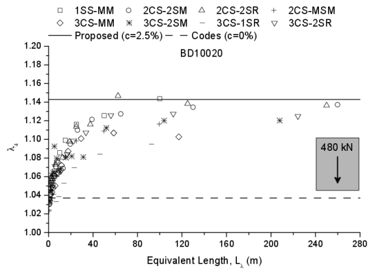
Fig. IV.35 \lambda_4 based on the proposed method for BD10020 traffic
