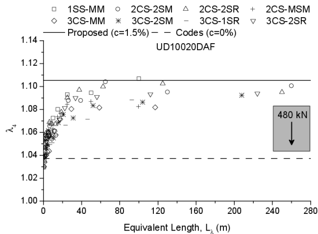
Fig. IV.40 \lambda_4 based on the proposed method for UD10020DAF traffic
