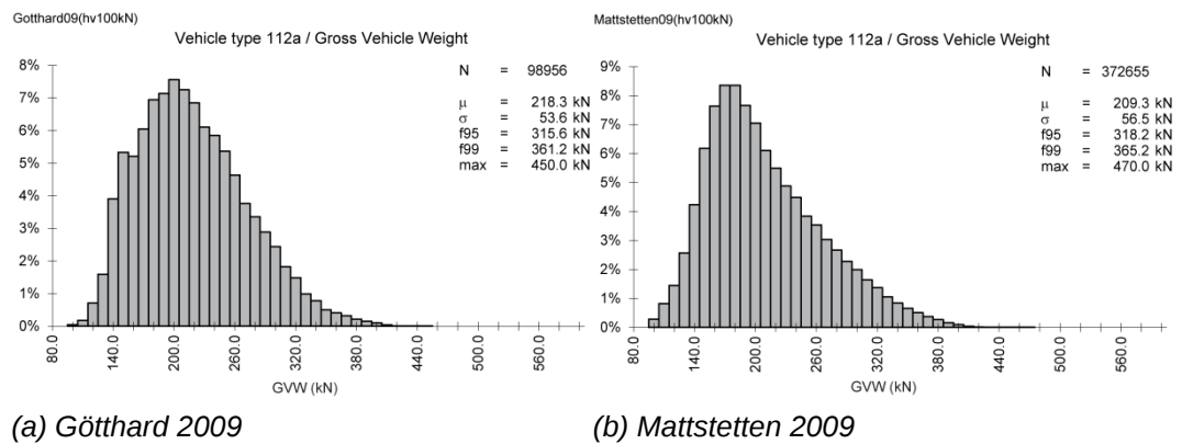
Fig. III.9 Frequency of GVW for truck Type 112a
