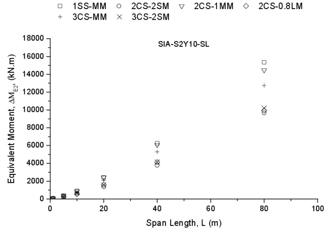
(a) Equivalent moment range
