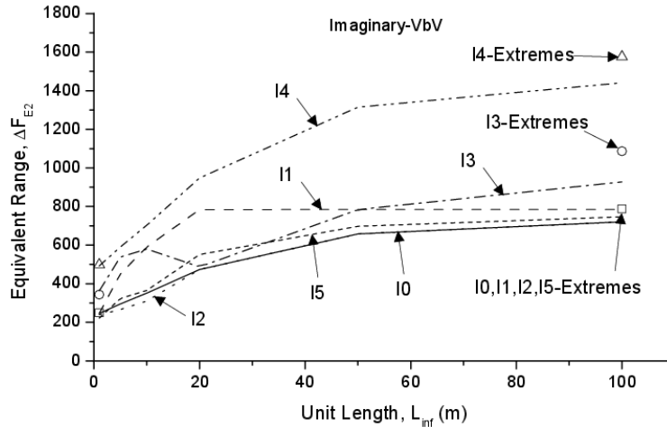
Fig. 4.3 Equivalent force range for imaginary influence lines
