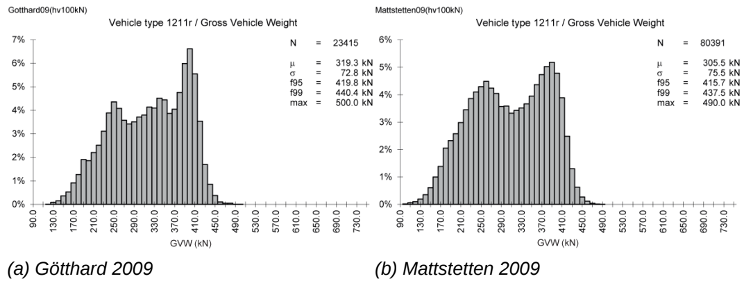
Fig. III.16 Frequency of GVW for truck Type 1211r
