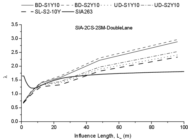
(b) Second support moment of two-span continuous bridges
