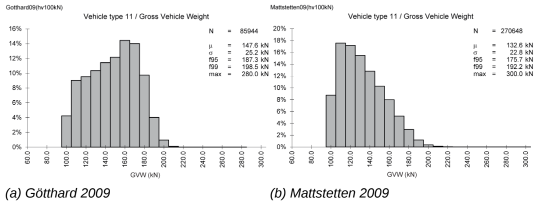
Fig. III.4 Frequency of GVW for truck Type 11
