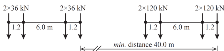
Fig. 3.7 Geometry of the fatigue load model (FLM3) taken from the EN1991-2 [25]
