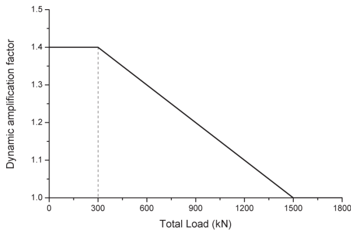
Fig. 2.15 Dynamic amplification factor in function of total load [51]
