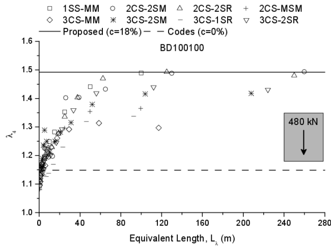
(a) bidirectional traffic, BD100100
