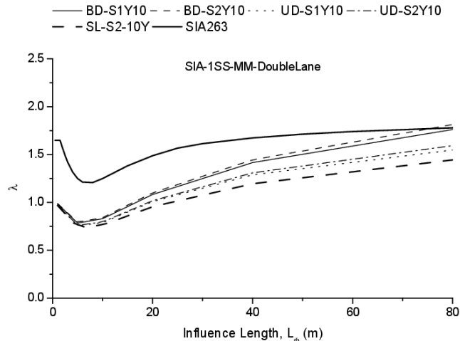
(a) Mid moment of simple-span bridges
