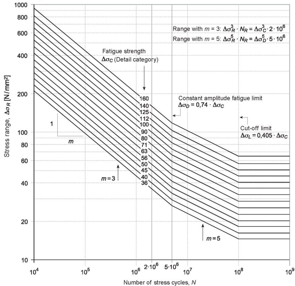
Fig. 2.5 Fatigue resistance and CAFL for different detail categories based on SIA263 [81]
