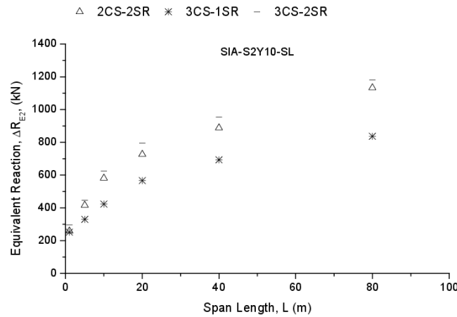
(b) Equivalent reaction range
