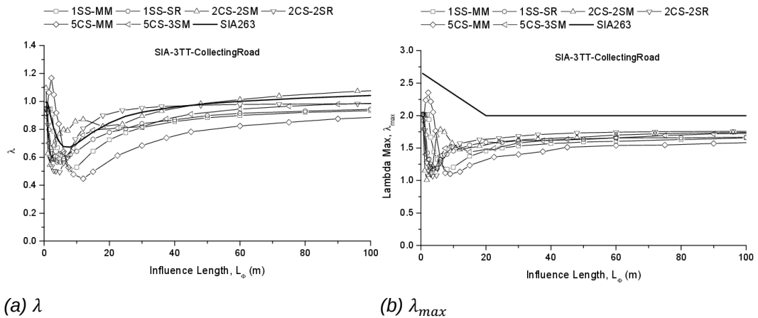
Fig. II.3 \lambda and \lambda_{max} obtained from 3TT for collecting road traffic in comparison with SIA263
