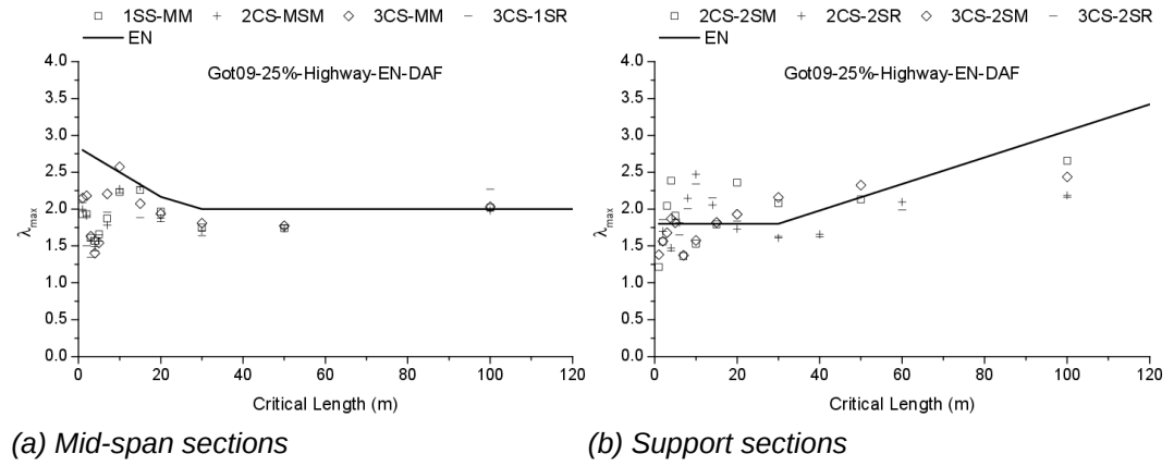
Fig. IV.17 Eurocode-base \lambda_{max} for G25HWDAF traffic
