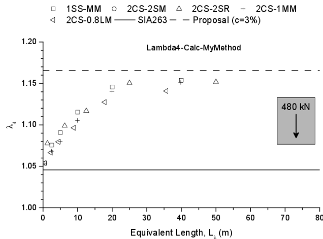
(b) Unidirectional traffic condition
