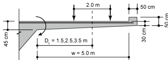
Fig. 4.21 Dimensions of studied cantilever slab and traffic lane position
