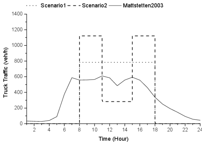
Fig. 3.12 Weekday truck traffic distribution of Mattstetten (2003), adapted to 2 \times 10^6 trucks/year/direction and two considered scenarios
