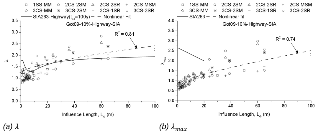
Fig. IV.1 SIA-base damage equivalence factors for G10HW traffic
