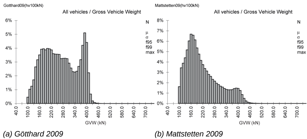
Fig. III.17 Frequency of GVW for all truck types
