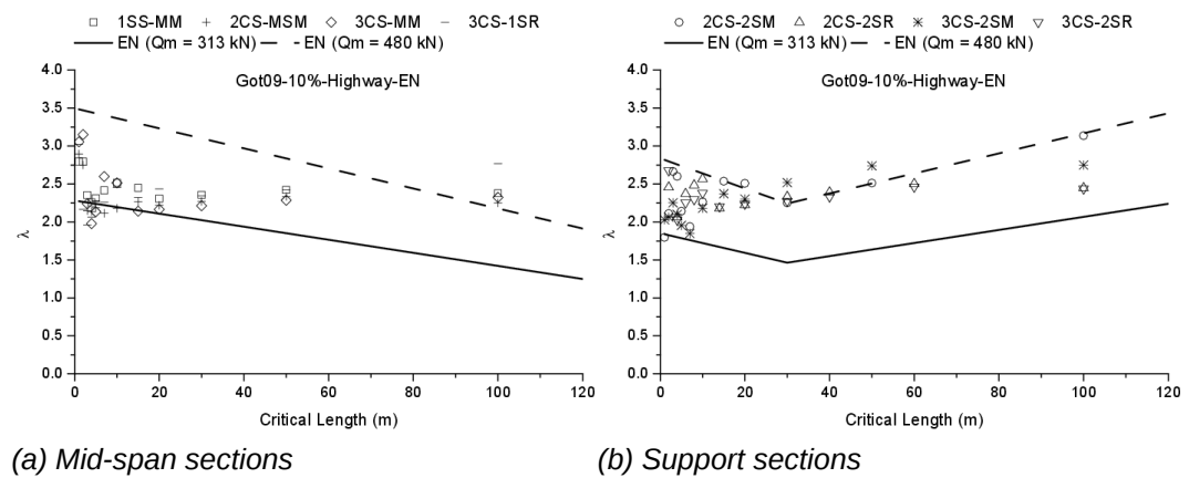
Fig. IV.7 Eurocode-base \lambda for G10HW traffic
