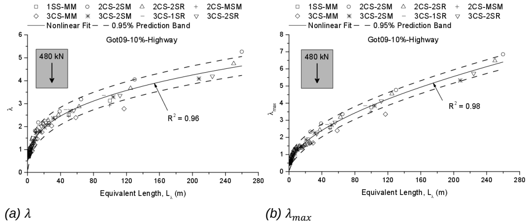
Fig. IV.19 \lambda and \lambda_{max} based on the proposed method obtained for G10HW traffic
