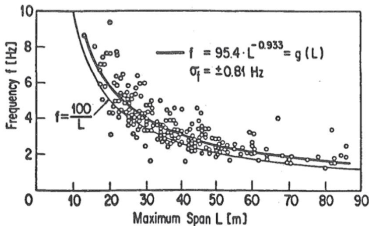
Fig. 2.13 Natural frequency versus span length, taken from [14]
