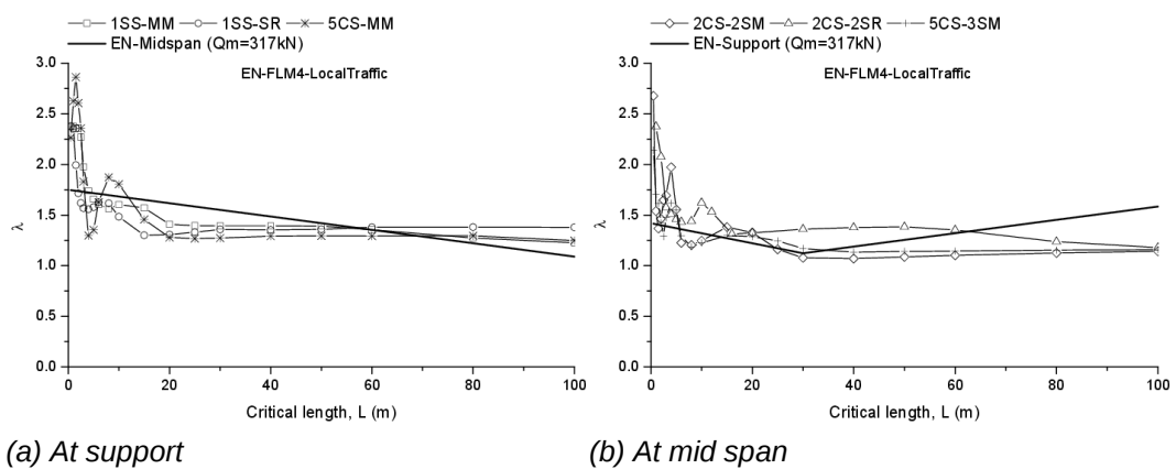
Fig. II.7 Comparison of \lambda with FLM4 for local traffic
