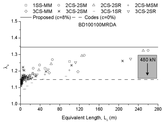
Fig. IV.42 \lambda_4 based on the proposed method for BD100100MRDAF traffic
