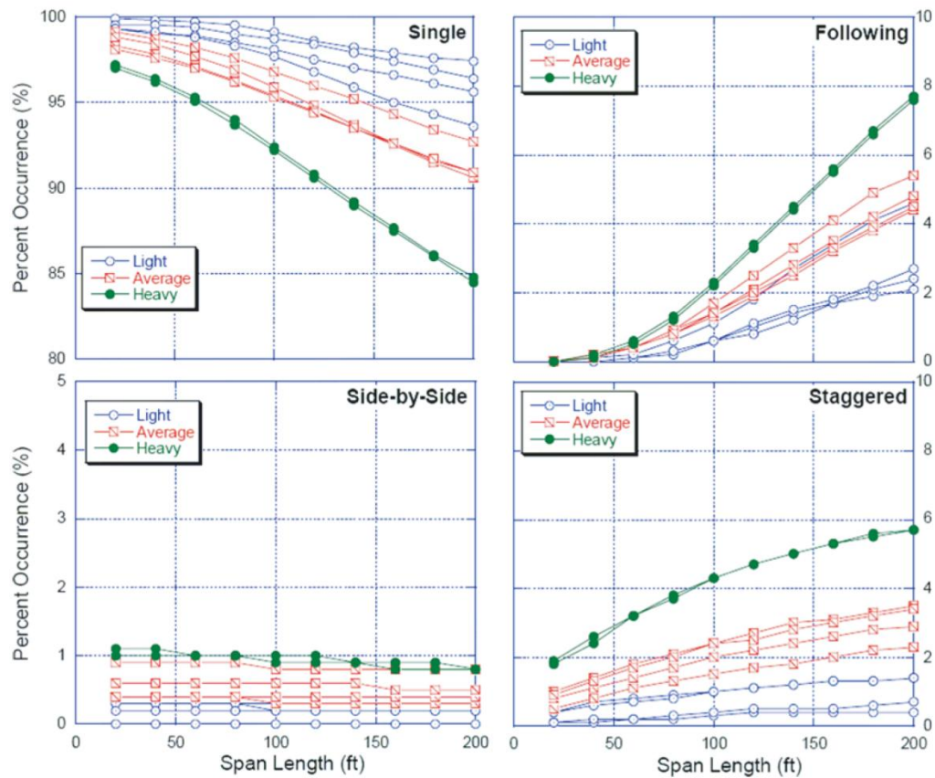
Fig. 2.12 Multiple presences frequencies for four loading patterns (1 ft = 30.5 cm) [83]
