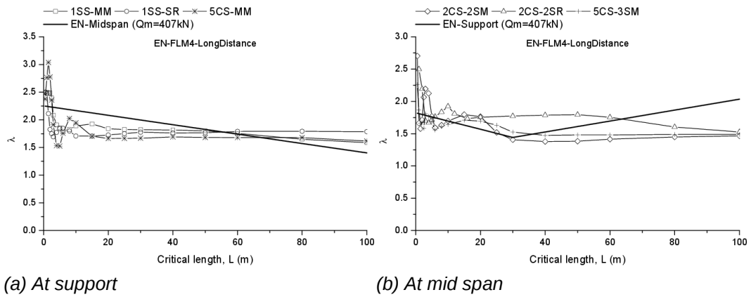
Fig. II.6 Comparison of \lambda with FLM4 for medium distance traffic
