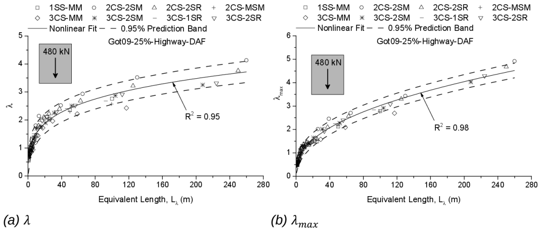
Fig. IV.23 \lambda and \lambda_{max} based on the proposed method obtained for G25HWDAF traffic
