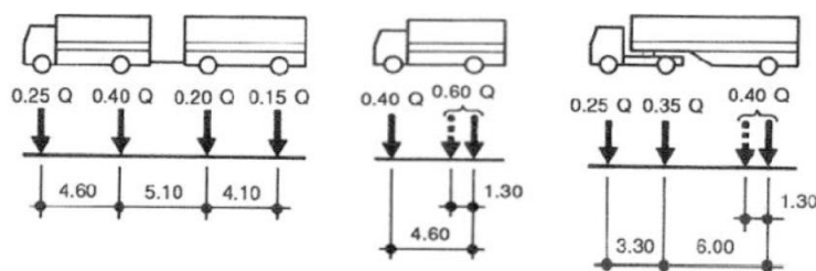
Fig. 3.5 Three truck types applied in development of the SIA codes [44]
