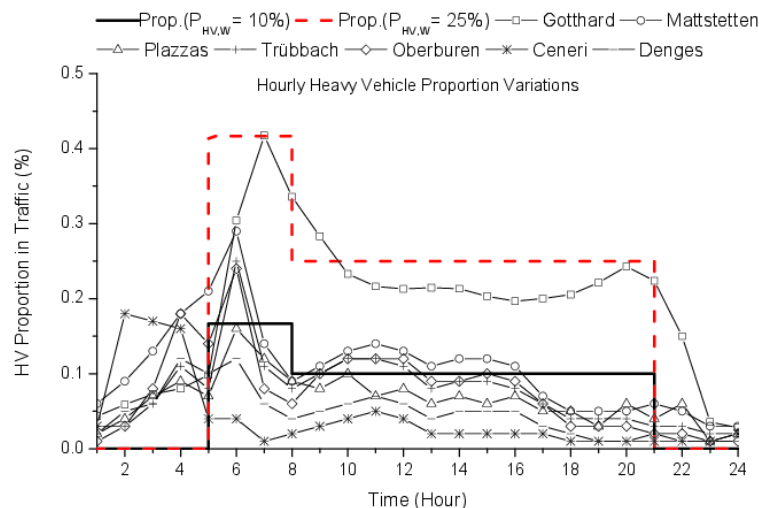
Fig. 5.4 Hourly Variations of Heavy Vehicles Proportion in Traffic (HVHVPT) of stations on weekdays and the proposed pattern
