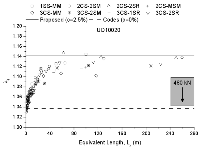
(b) unidirectional traffic, UD10020
