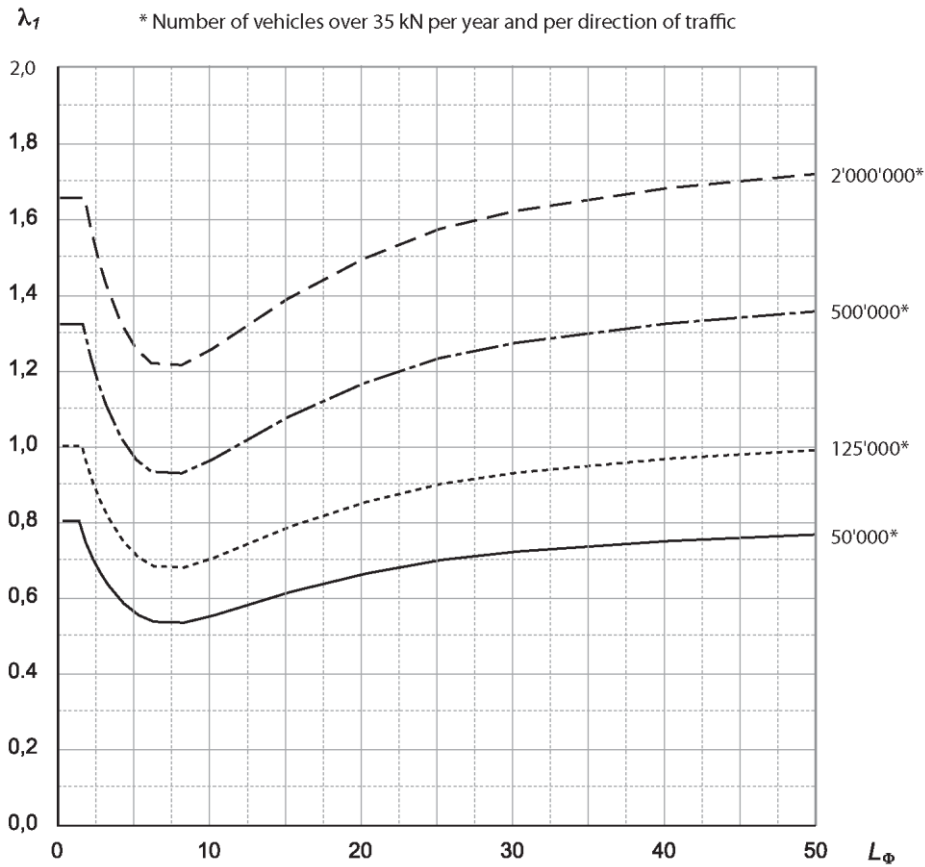
Fig. 3.2 \lambda_1 for roadway bridge with different traffic volumes, taken and modified from the SIA261 [80]
