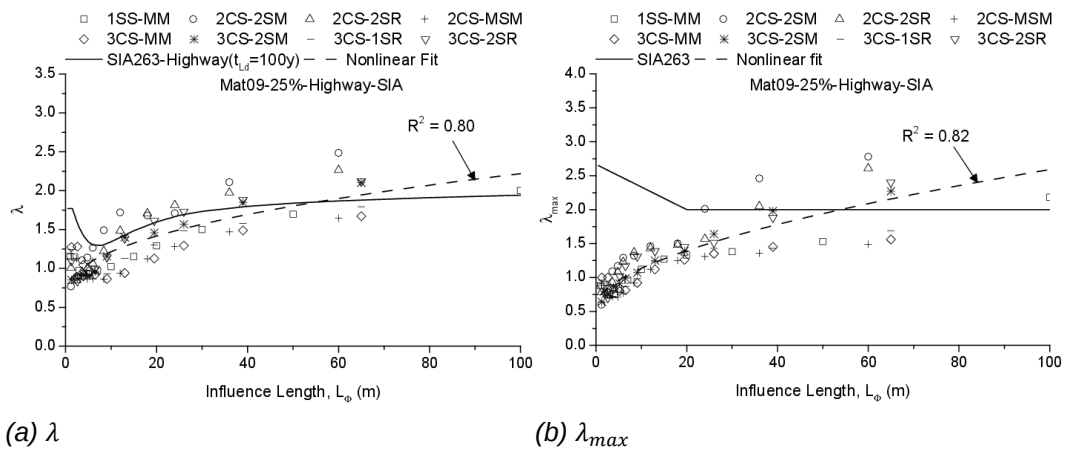
Fig. IV.4 SIA-base damage equivalence factors for M25HW traffic
