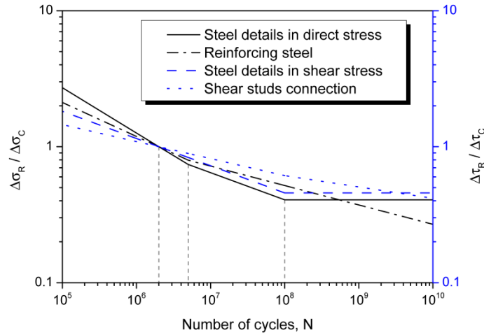
Fig. 6.12 Samples of S-N curves for different details
