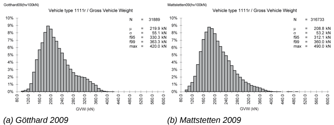
Fig. III.14 Frequency of GVW for truck Type 1111r
