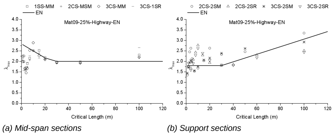
Fig. IV.16 Eurocode-base \lambda_{max} for M25HW traffic
