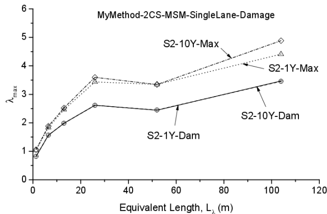
(b) Mid-support moment of two-span bridges
