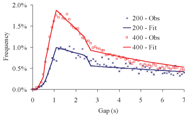
Fig. 2.10 Trucks time intervals distributions at two flow rates [28]
