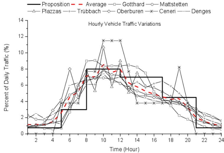
Fig. 5.3 Normalized Hourly Traffic Variations (HTV) of stations on weekdays and the proposed pattern
