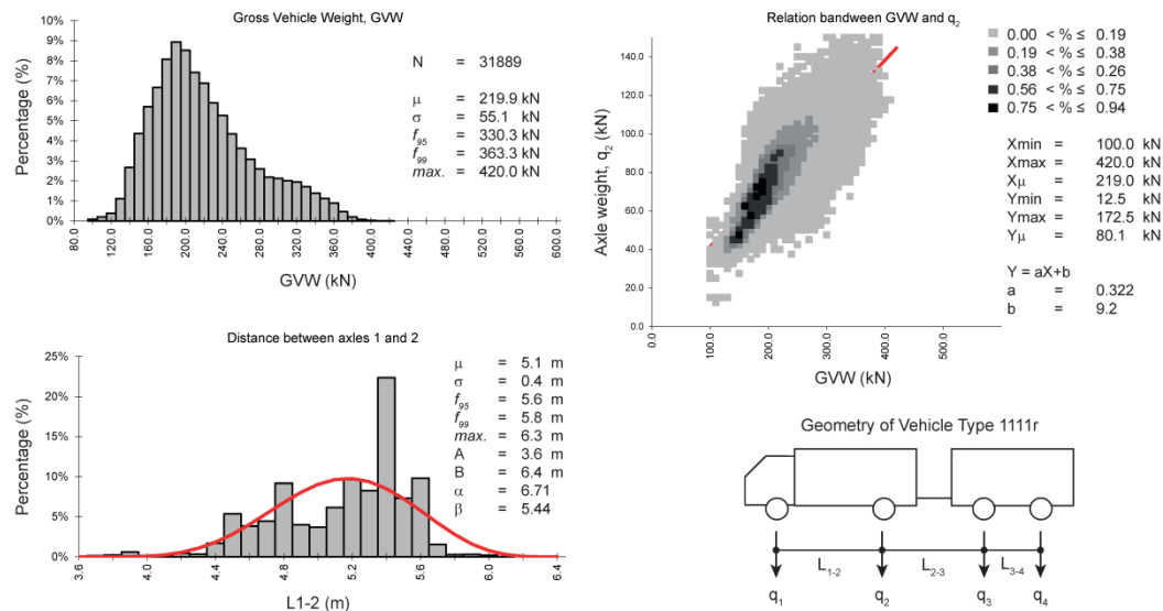
Fig. III.3 Sample of statistical analysis of data from Götthard traffic database
