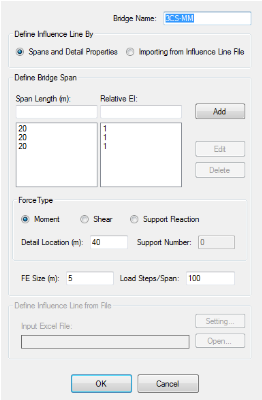
(c) Bridge definition dialog box
