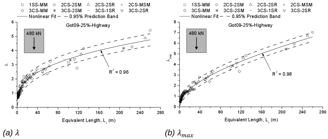
Fig. IV.20 \lambda and \lambda_{max} based on the proposed method obtained for G25HW traffic
