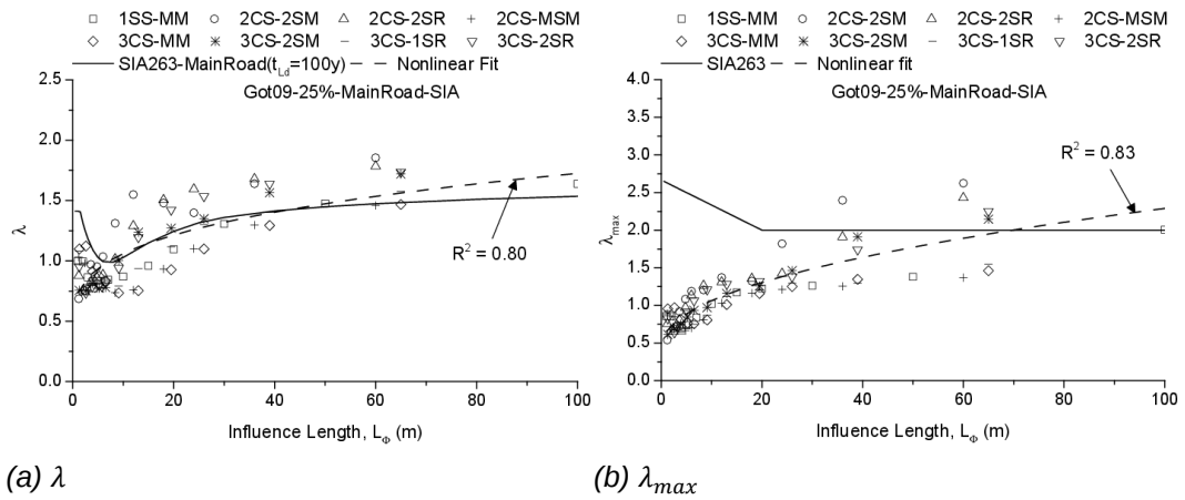
Fig. IV.3 SIA-base damage equivalence factors for G25MR traffic
