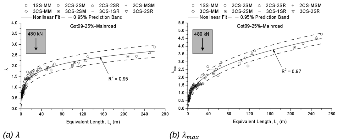
Fig. IV.21 \lambda and \lambda_{max} based on the proposed method obtained for G25MR traffic
