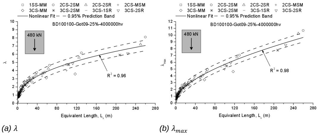
Fig. IV.26 \lambda and \lambda_{max} based on the proposed method obtained for BD100100 traffic
