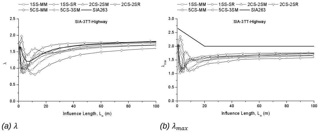
Fig. II.1 \lambda and \lambda_{max} obtained from 3TT for highway traffic in comparison with SIA263
