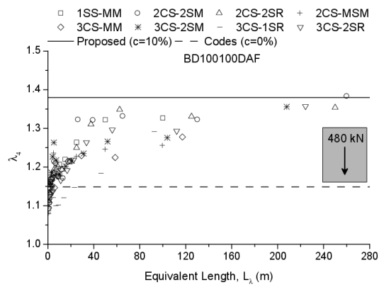
Fig. IV.41 \lambda_4 based on the proposed method for BD100100DAF traffic
