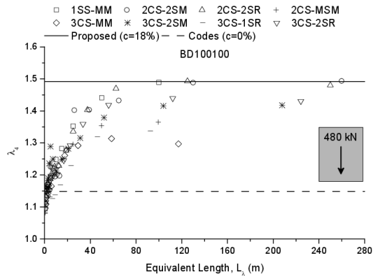
Fig. IV.34 \lambda_4 based on the proposed method for BD100100 traffic
