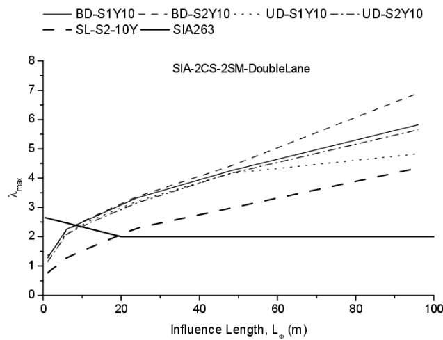
(b) Two-span continuous bridge - second support moment
