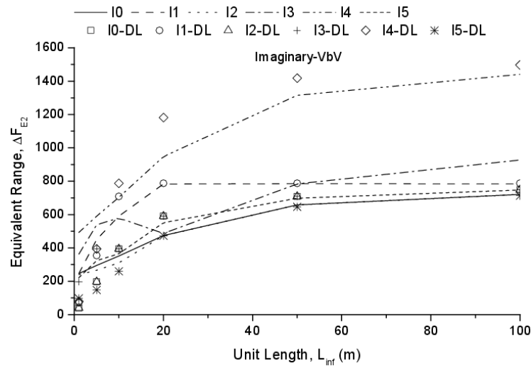
Fig. 4.11 Equivalent force range estimated by uniformly distributed load in comparison with simulations
