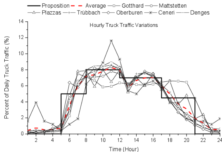
Fig. 5.2 Normalized Hourly Truck Traffic Variations (HTTV) of the stations on weekdays and the proposed pattern
