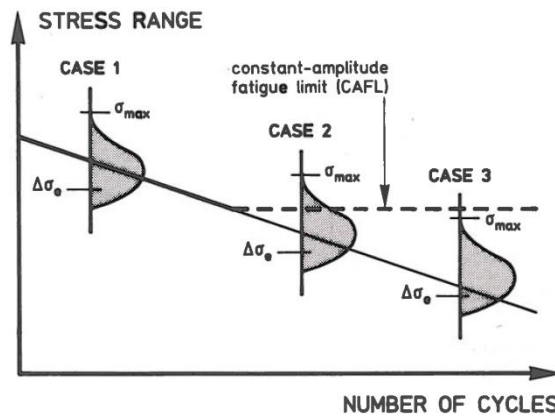
Fig. 2.3 Three cases of variable amplitude stress spectra [84]
