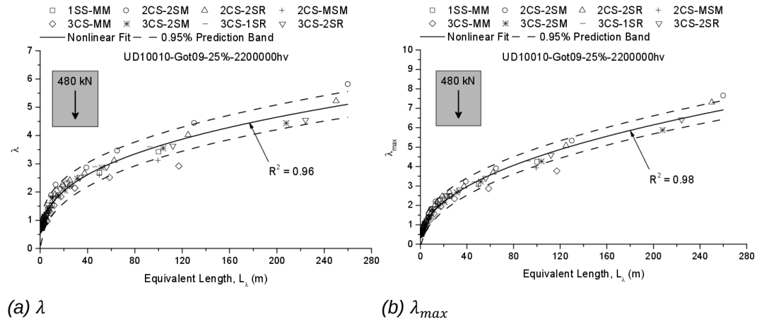
Fig. IV.28 \lambda and \lambda_{max} based on the proposed method obtained for UD10010 traffic
