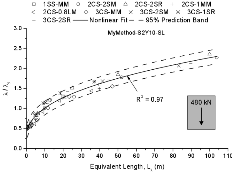
Fig. 4.15 \lambda for different influence lines based on the proposed method
