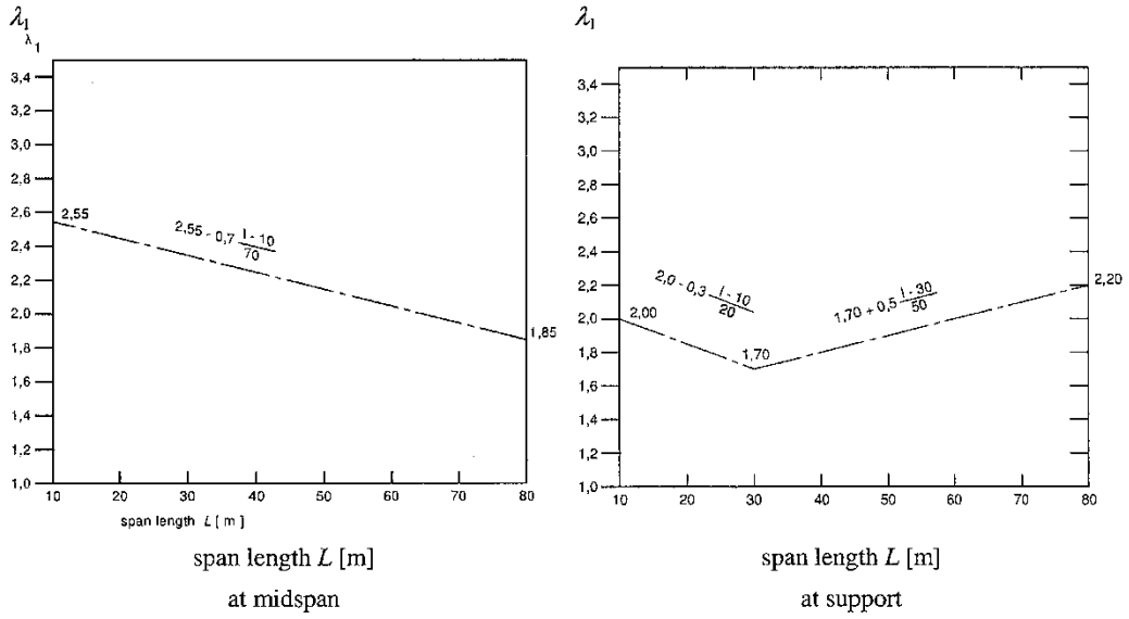
Fig. 3.8 \lambda_1 for roadway bridges based on EN1993-2 [27]
