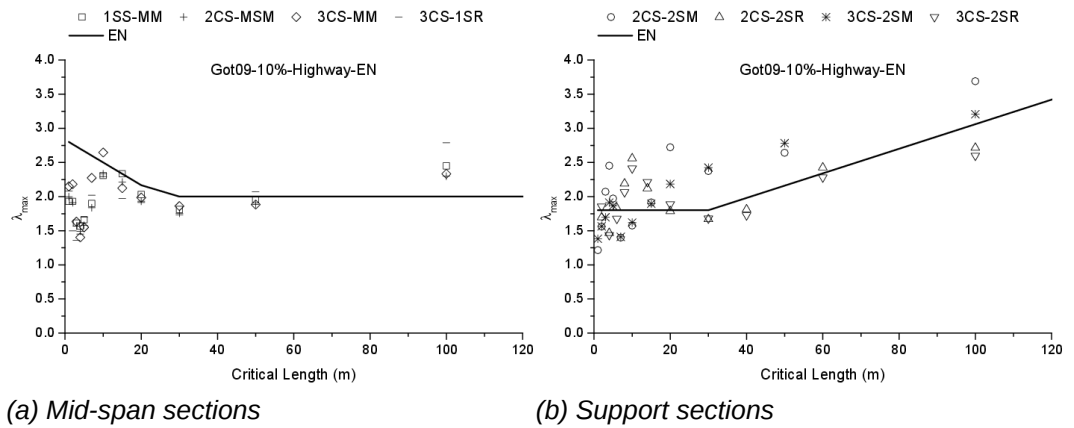
Fig. IV.13 Eurocode-base \lambda_{max} for G10HW traffic
