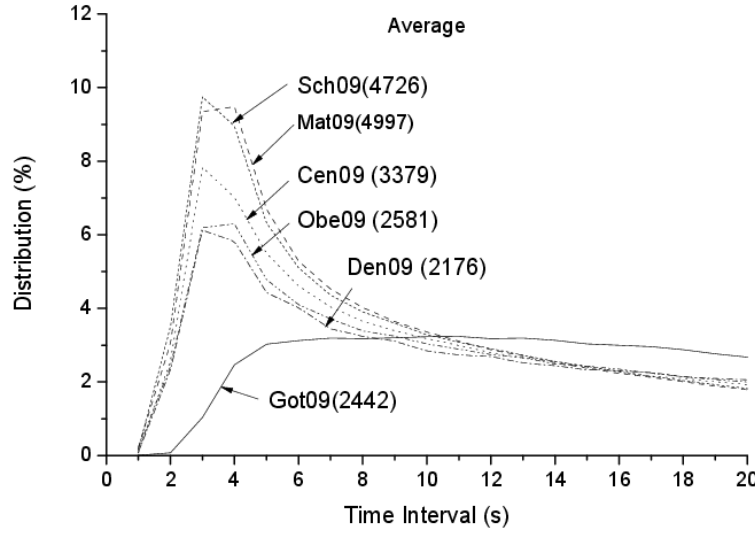
Fig. 4.12 Frequency of time intervals between heavy vehicles for different WIM stations of Switzerland in 2009
