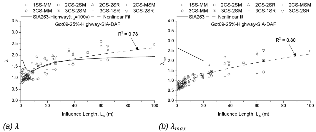
Fig. IV.5 SIA-base damage equivalence factors for G25HWDaf traffic
