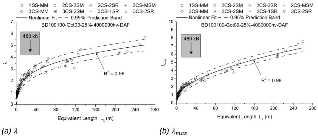
Fig. IV.32 \lambda and \lambda_{max} based on the proposed method obtained for BD100100DAF traffic
