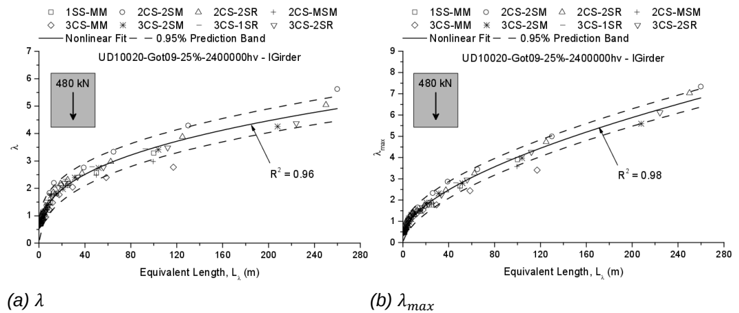
Fig. IV.30 \lambda and \lambda_{max} based on the proposed method obtained for UD10020IG traffic
