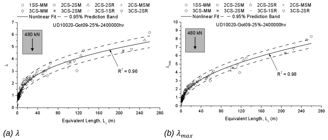
Fig. IV.29 \lambda and \lambda_{max} based on the proposed method obtained for UD10020 traffic
