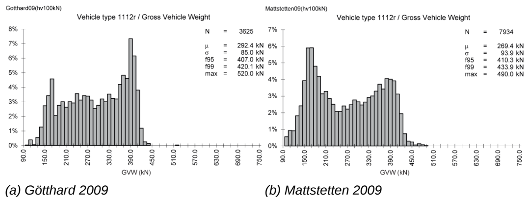
Fig. III.15 Frequency of GVW for truck Type 1112r
