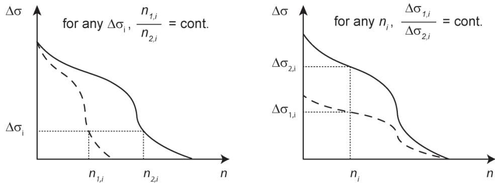
(a) Proportional in number of cycles
