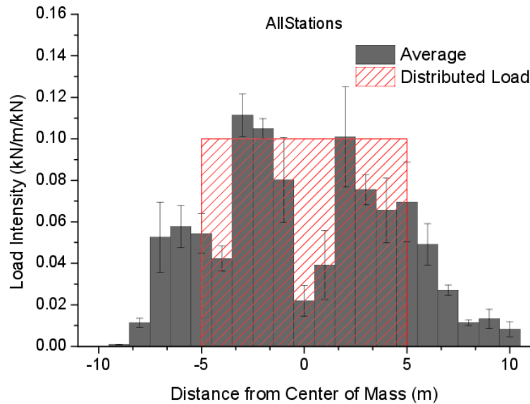
Fig. 4.8 Average equivalent vehicle and its standard deviation obtained for Swiss traffic
