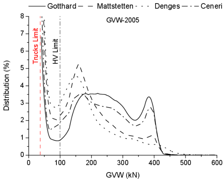
Fig. 5.5 GVW distribution of some WIM stations measured in 2005
