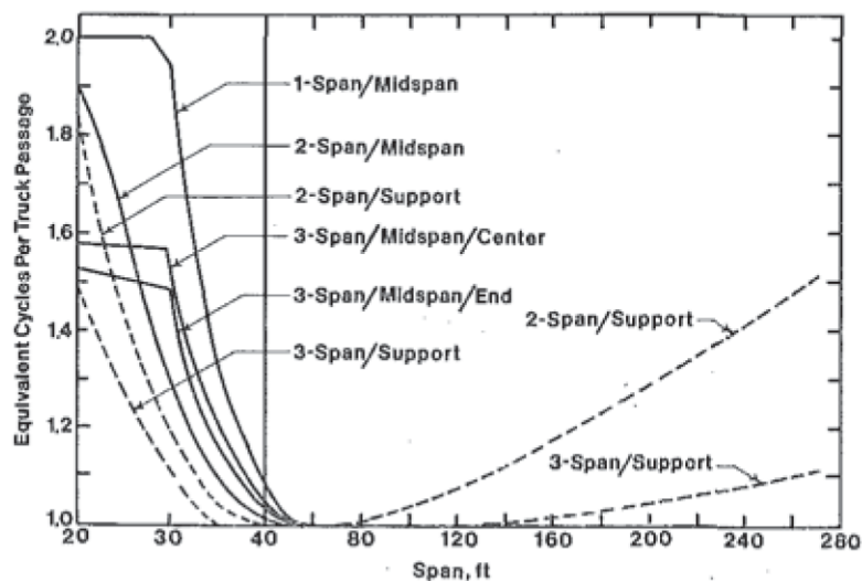
Fig. 2.6 Equivalent cycles per truck passage as a function of span (1 ft = 30.5 cm) [75]
