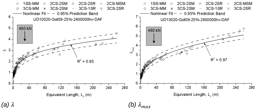
Fig. IV.31 \lambda and \lambda_{max} based on the proposed method obtained for UD10020DAF traffic
