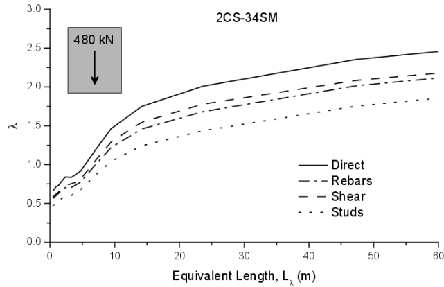
(a) Two-span continuous bridge, 3/4 span length moment
