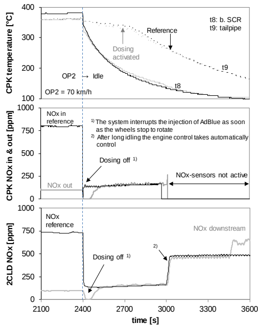
Fig. 11: SWOFF – ECU intervention after long idling period. OEM SCR; dosing OP2 activated; Vehicle D; ULSD, chassis dyno LARAG
