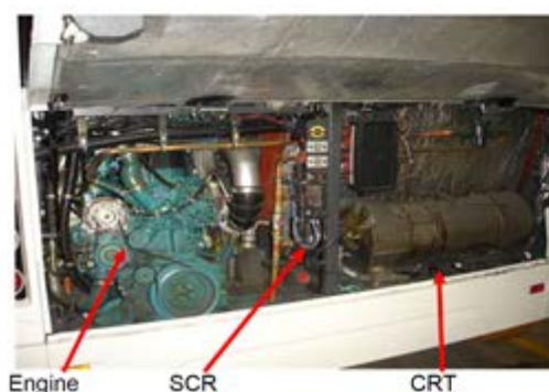
Combustion engine and CRT + SCR -System
