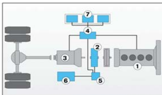
The drive-train of Volvo 7700 Hybrid Bus
