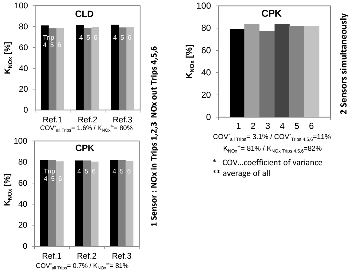
Fig. 8: Comparison of KNO x -dispersion between 2 measurement types: with 1 sensor only and with 2 sensors simultaneously. Periods of active SCR & CPK sensors; vehicle F; ULSD; AdBlue; dosing activated.
